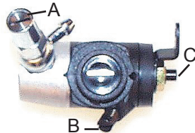
Rotary Carburetor
