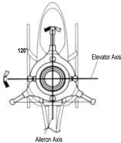
120° Three-Servo CCPM Control System
