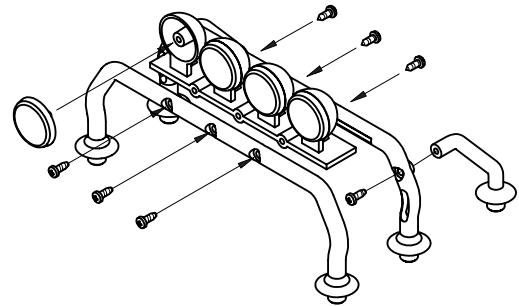
❑ 3. Assemble the rollbar as shown using ten 2.6 x 6mm self-tapping screws.
