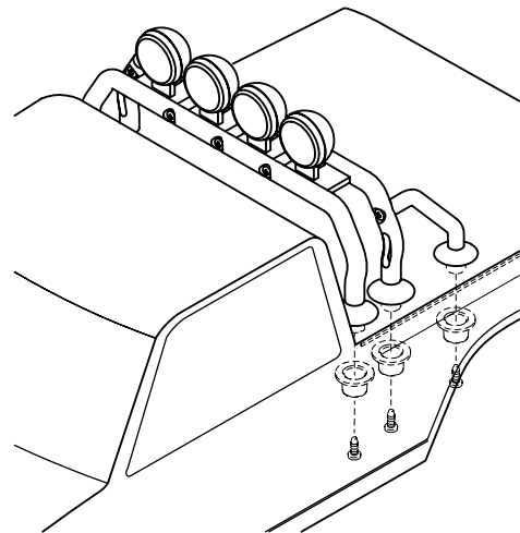
❑ 4. Drill six 1/4" (6mm) holes in the body using the molded-in dimples as guides. Install the rollbar onto body as shown using six 2.6 x 6mm self-tapping screws and the included collars.
